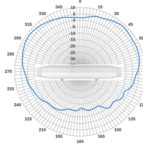
CW9178I – 2.4 GHz Radio Antenna Pattern
